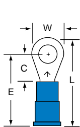
MV14-10R Stud Size 10 Wire Range 16-14
