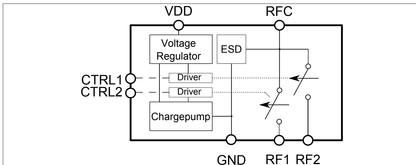
Figure 1: BGSA11GN10 block diagram
