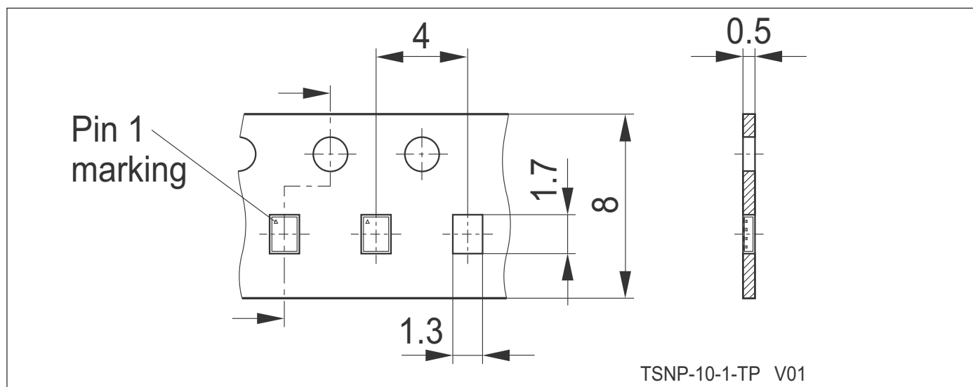
Figure 5: Tape drawing
