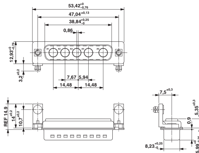
Dimensioned drawing
