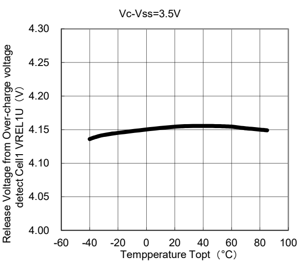
4) Release Voltage from Over-charge (Cell1) vs. Temperature R5460x201AC
