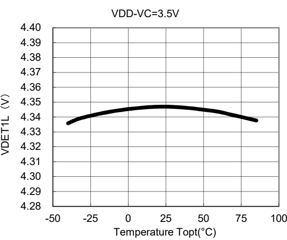
3) Over-Charge Voltage Threshold (Cell2) vs. Temperature R5460x201AC
