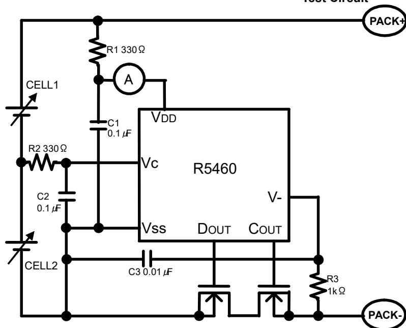
Test Circuit
