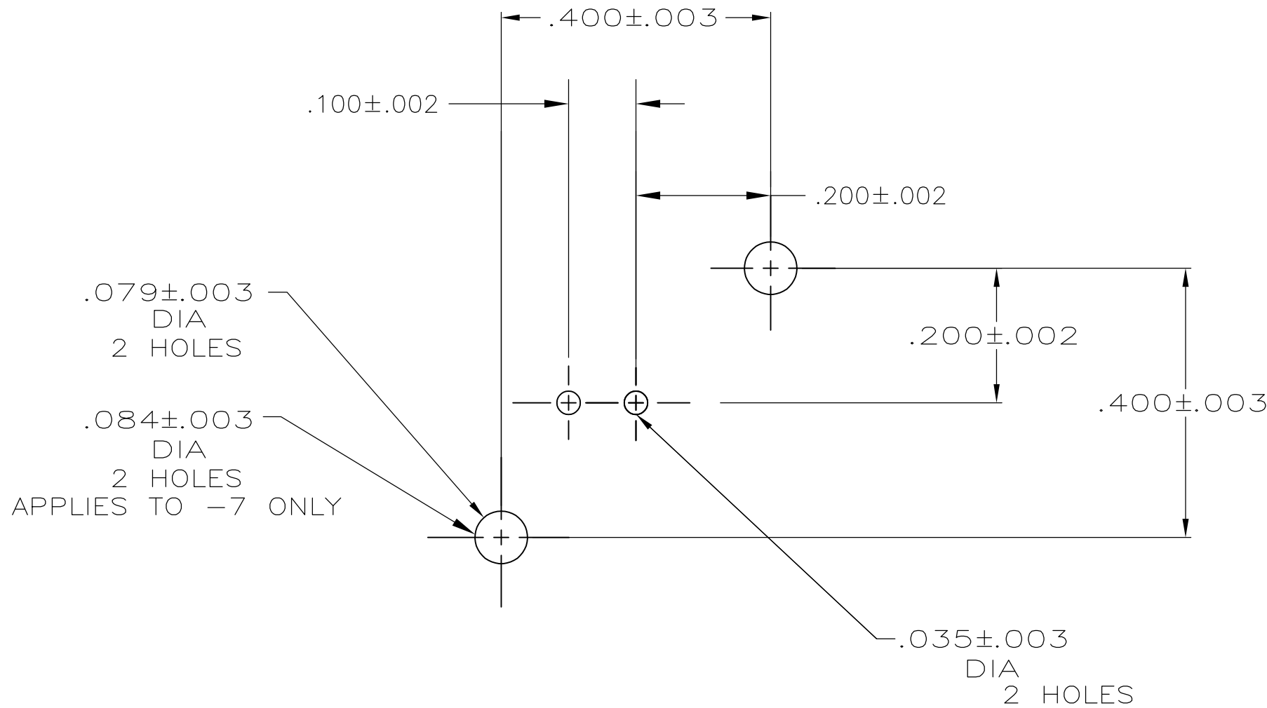
PCB CONFIGURATION
