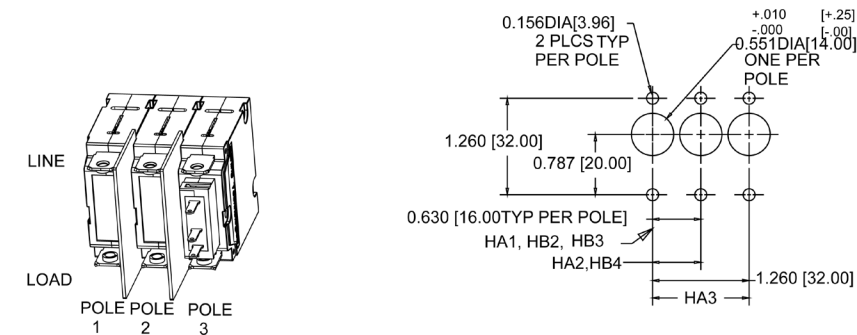
PANEL CUTOUT DETAIL
