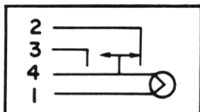
Typical 4 Terminal Press-To-Switch Circuit
