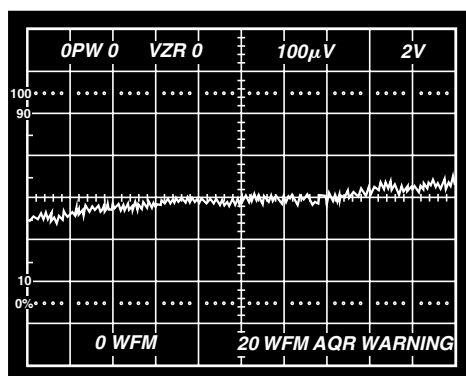
TPC 26. Gain Nonlinearity, G = 100 , R_L = 10 k\Omega , C_L = 0 pF . Vertical Scale: 100 \mu V /Div = 100 ppm/Div Horizontal Scale: 2 Volts/Div
