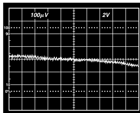
TPC 27. Gain Nonlinearity, G = 10 , R_L = 10 k\Omega , Vertical Scale: 100 \mu V /Div = 100 ppm/Div, Horizontal Scale: 2 Volts/Div
