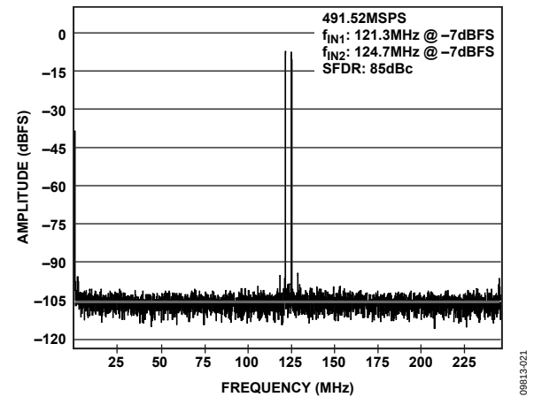
Figure 21. 16k Point Single-Tone FFT; 491.52 MSPS, f_{IN1} = 121.3 MHz, f_{IN2} = 124.7 MHz
