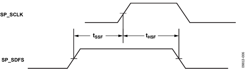
Figure 6. Slave Mode SP_SDFS Setup/Hold Time
