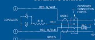
SCHEMATIC DIAGRAM
