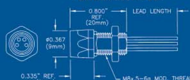
FEMALE RECEPTACLE
