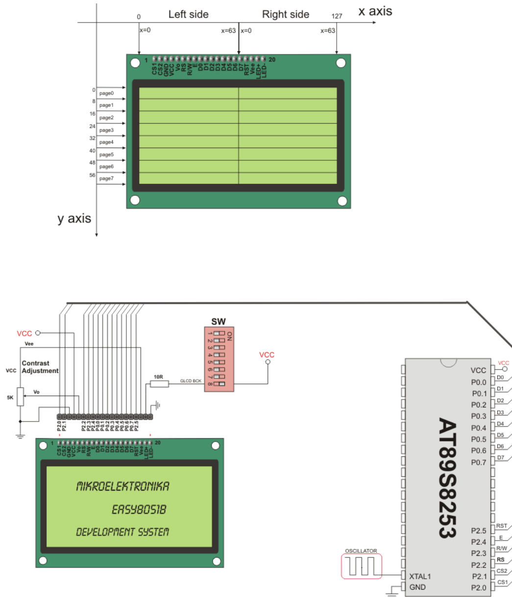
GLCD HW connection
