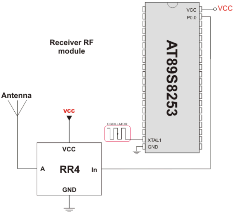
Simple Receiver connection
