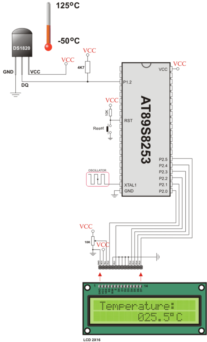
Example of DS1820 connection
