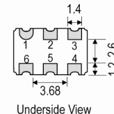
Underside View
