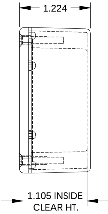
DETAIL D SCALE 6 : 1
