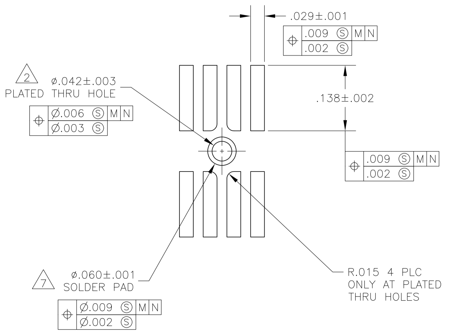
DETAIL G SCALE 8:1
