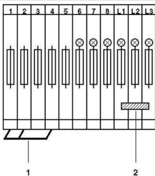
Circuit diagram
