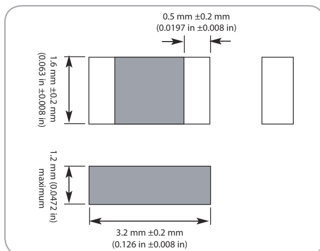
NTC Type NHQ Outline Drawing
