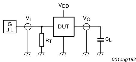
Test data is given in Table 10 . Definitions for test circuit: C_L = Load capacitance including jig and probe capacitance. R_T = Termination resistance should be equal to output impedance Z_o of the pulse generator.
