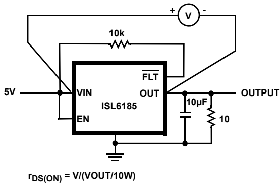
FIGURE 29A. r DS(ON)
