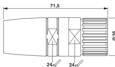
Dimensional drawing
