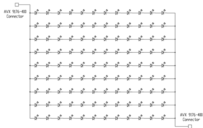
Figure 15: Electrical circuit diagram for L235-xyyyAML5WAD0.
