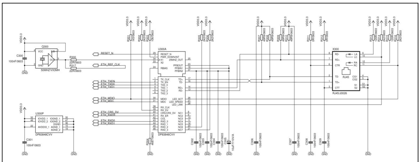
Figure 3 Ethernet Interface
