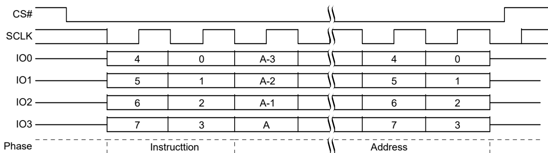
Figure 85. Block Erase (BE D8h or 4BE DCh) QPI Mode Command Sequence
