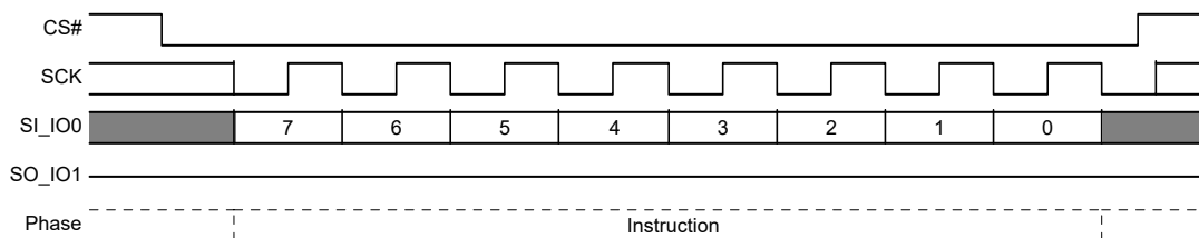
Figure 47. Clear Status Register (CLSR) Command Sequence
