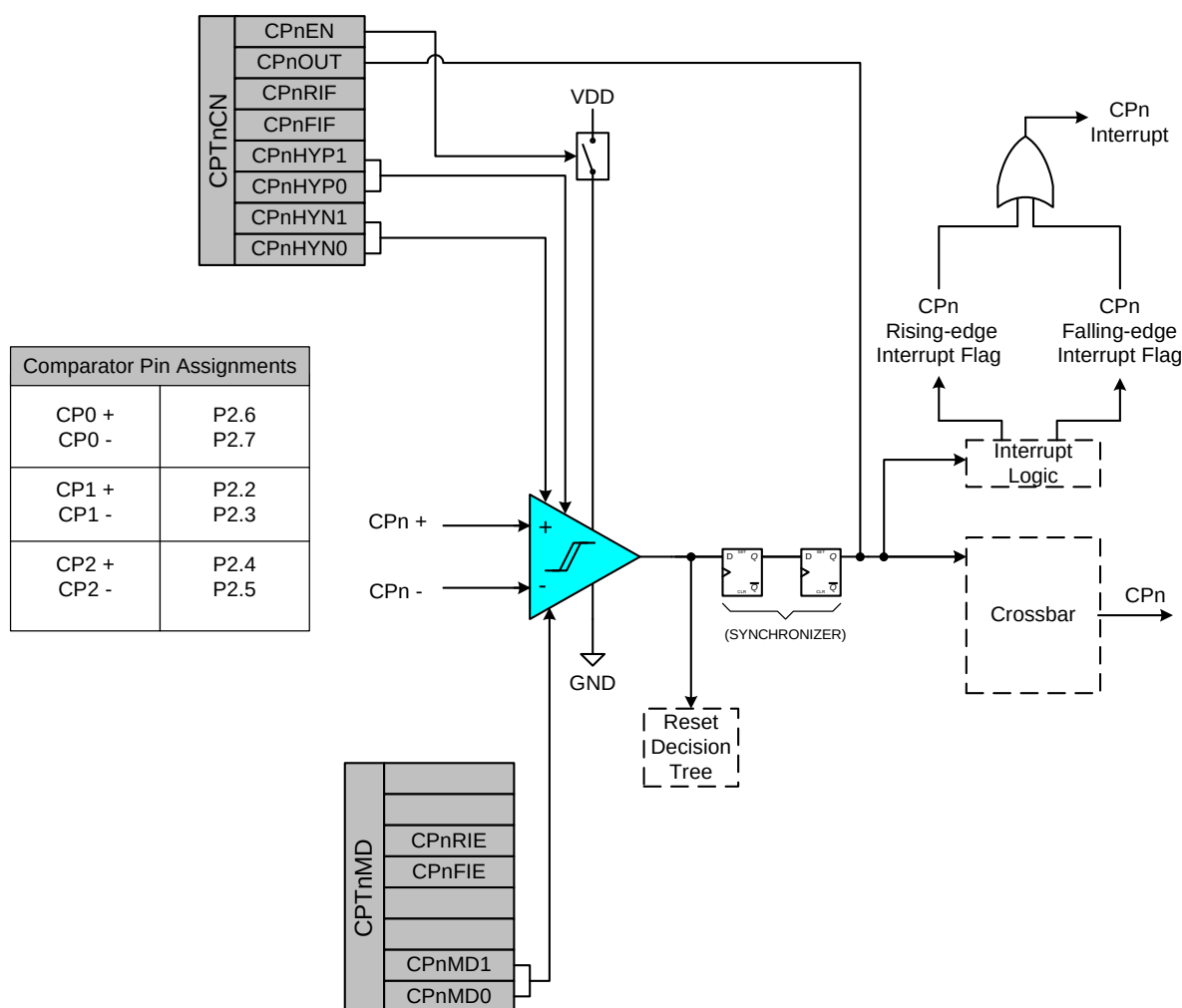
Figure 12.1. Comparator Functional Block Diagram
