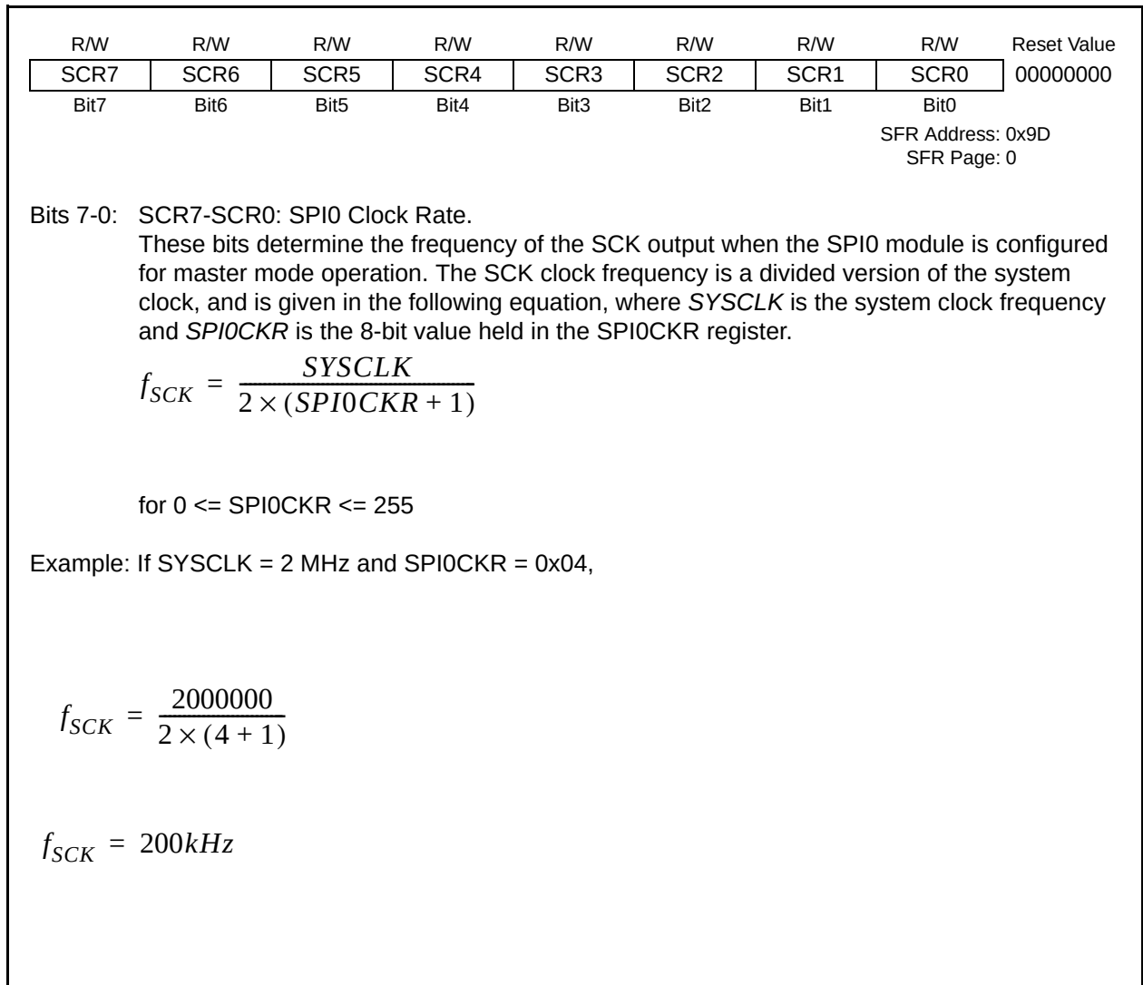
Figure 21.10. SPI0CKR: SPI0 Clock Rate Register
