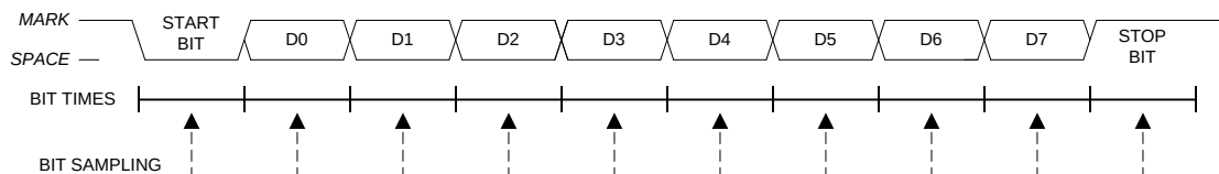
Figure 23.4. 8-Bit UART Timing Diagram
