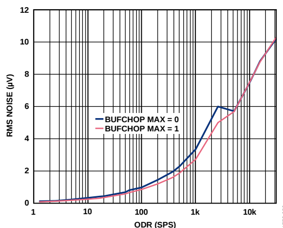
Figure 52. RMS Noise vs. Output Data Rate (Sinc5 + Sinc1 Filter)
