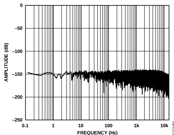
Figure 51. Shorted Input FFT
