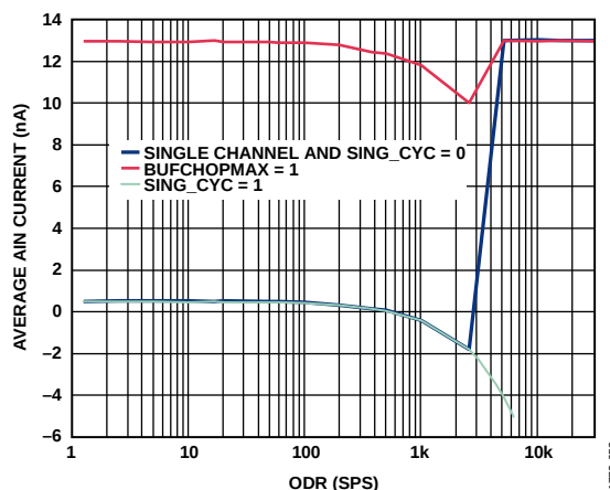
Figure 53. Typical Analog Input Current vs. Output Data Rate (2.5 V Common Mode)
