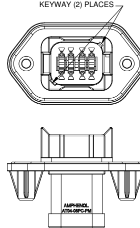
P/N AT04-08PC-PMXX KEY-C CONFIGURATION STANDARD COLOR: GREEN
