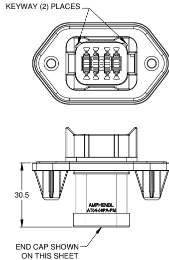
P/N AT04-08PA-PMXX KEY-A CONFIGURATION STANDARD COLOR: GREY
