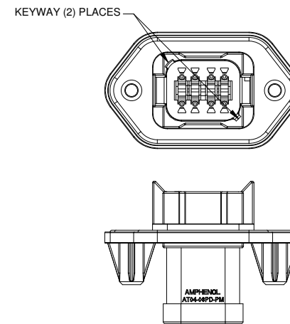
P/N AT04-08PD-PMXX KEY-D CONFIGURATION STANDARD COLOR: BROWN
