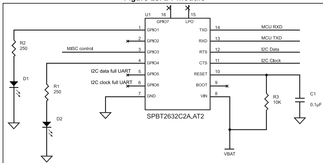
Figure 13. BT module
