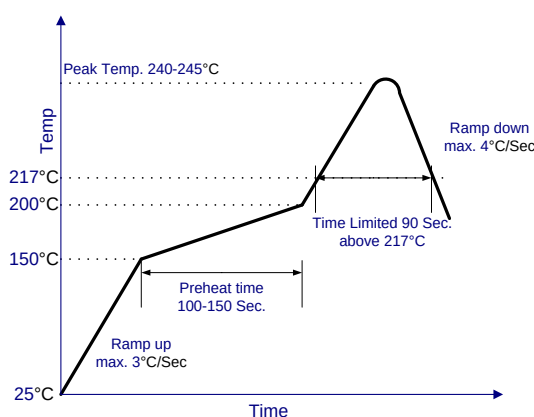
Figure 39. Recommended linear reflow profile using Sn/Ag/Cu solder.
