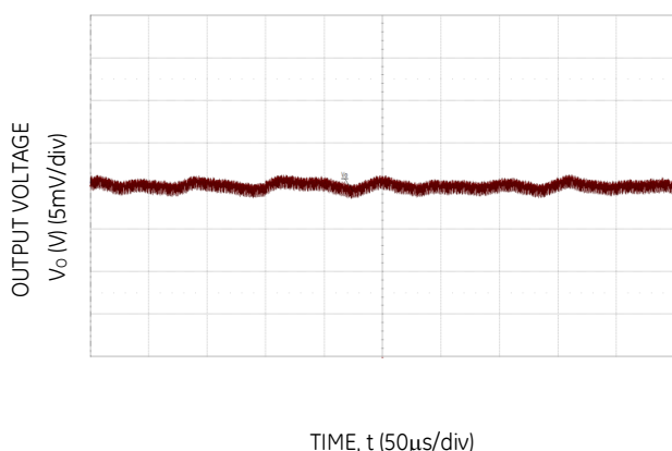
Figure 9. Typical output ripple and noise (C o =12x47μF ceramic + 10x470μF polymer, V IN = 12V, I o = I o,max )
