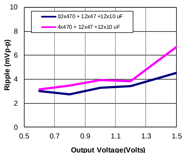
Figure 32. Peak to peak output ripple voltage for various output voltages with external capacitors at the output (170A load). Input voltage is 12V.
