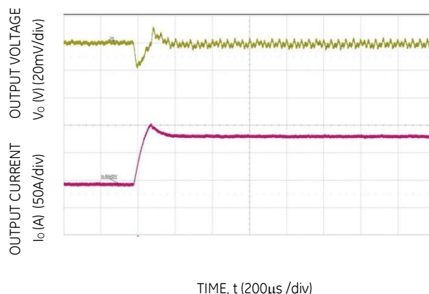
Figure 10. Transient Response to Dynamic Load Change from 25% to 75% at 12Vin, C o = 12 x 47μF + 10 x 1000μF, R TUNE = 3.01kΩ.
