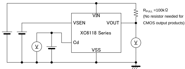
Circuit 9
