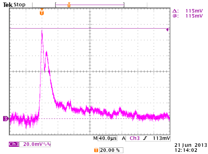
FIGURE 11. (5 - 3 A) LOAD STEP, di/dt = 2.5\text{ A}/\mu\text{s}
