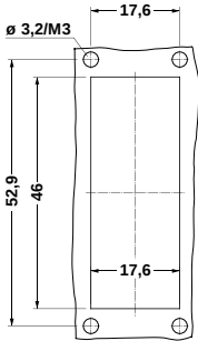
Panel cutout: VS-15-A-GC...
