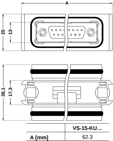
Dimensional drawing: VS-15-KU...
