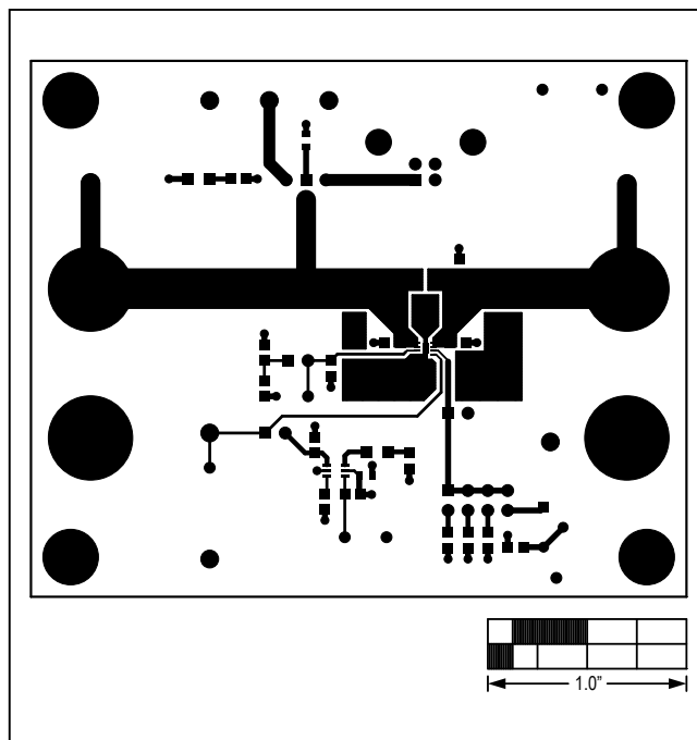
Figure 3. MAX14575A–MAX14575C EV Kit PCB Layout—Component Side
