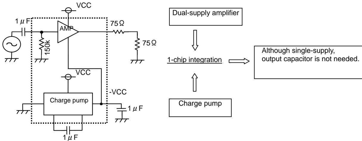
Fig.6 Configuration Diagram of BH769xxGU or BH76706GU
