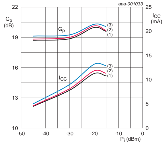
T_{amb} = 25 \text{ }^\circ\text{C}; f = 1575 \text{ MHz}. (1) V_{CC} = 1.5 \text{ V} (2) V_{CC} = 1.8 \text{ V} (3) V_{CC} = 2.2 \text{ V}
