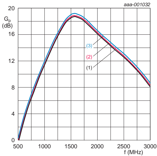
P_i = -45 \text{ dBm}; T_{amb} = 25 \text{ }^\circ\text{C}. (1) V_{CC} = 1.5 \text{ V} (2) V_{CC} = 1.8 \text{ V} (3) V_{CC} = 2.2 \text{ V}
