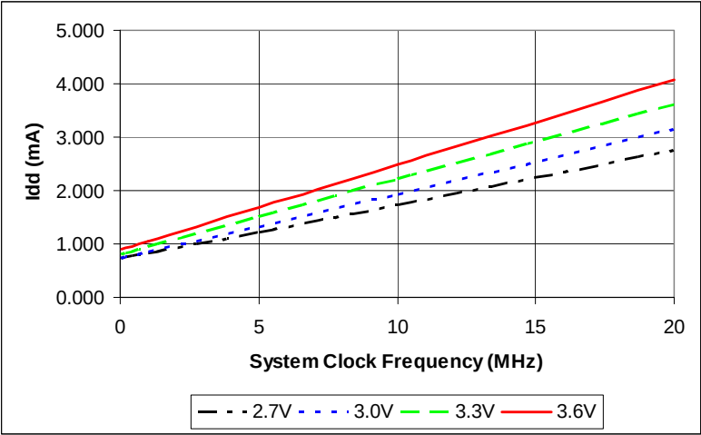
Figure 44. Maximum HALT Mode I_{CC} vs. System Clock Frequency
