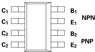
PARTMARKING DETAIL – T6718
