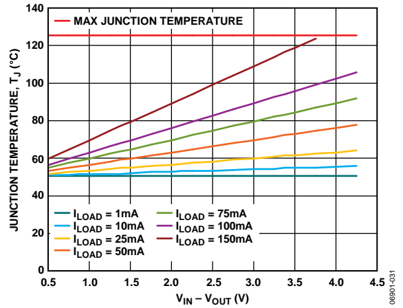
Figure 37. TSOT, 500 mm 2 of PCB Copper, T_A = 50^\circ C
