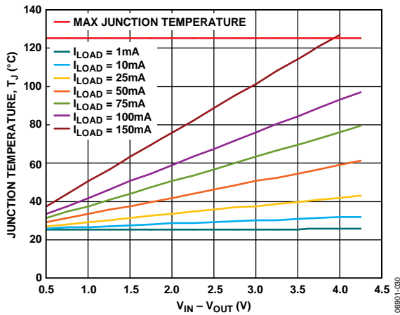
Figure 36. TSOT, 0 mm 2 of PCB Copper, T_A = 25^\circ C
