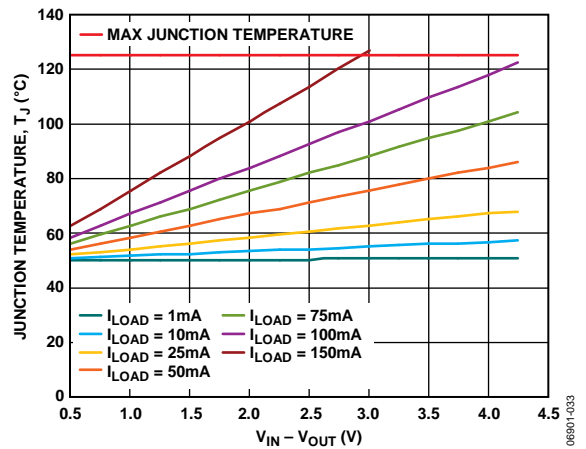
Figure 39. TSOT, 0 mm 2 of PCB Copper, T_A = 50^\circ C
