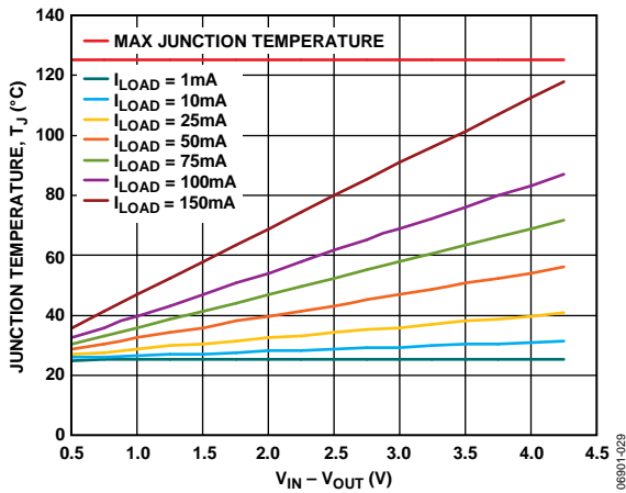
Figure 35. TSOT, 100 mm 2 of PCB Copper, T_A = 25^\circ C
