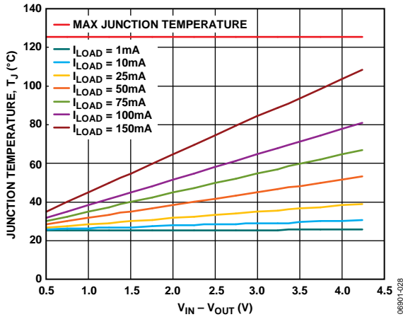
Figure 34. TSOT, 500 mm 2 of PCB Copper, T_A = 25^\circ C
