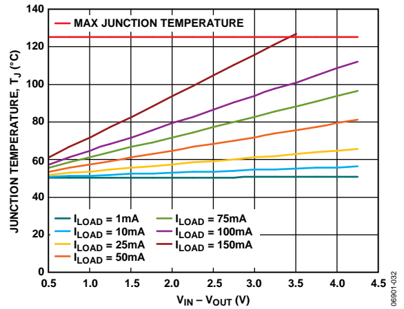
Figure 38. TSOT, 100 mm 2 of PCB Copper, T_A = 50^\circ C
