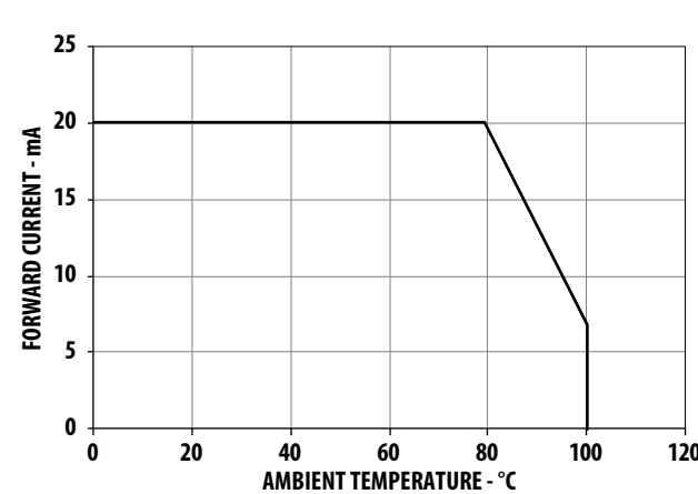
Figure 4: Ambient Temperature vs. Maximum DC Forward Current
