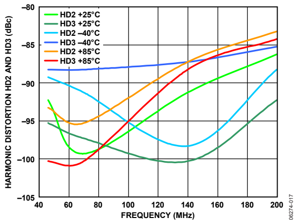
Figure 18. Harmonic Distortion vs. Frequency, Three Temperatures, V_{OUT} = 2 V p-p
