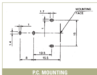
P.C. MOUNTING
