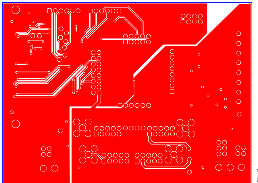
Figure 13. EVAL-MBnanoDAC-SDZ Motherboard Bottom Side Routing
