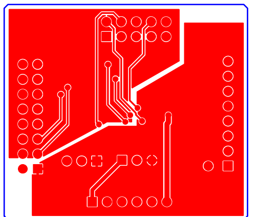
Figure 17. EVAL-AD5341DBZ Daughter Board Bottom Side Routing
