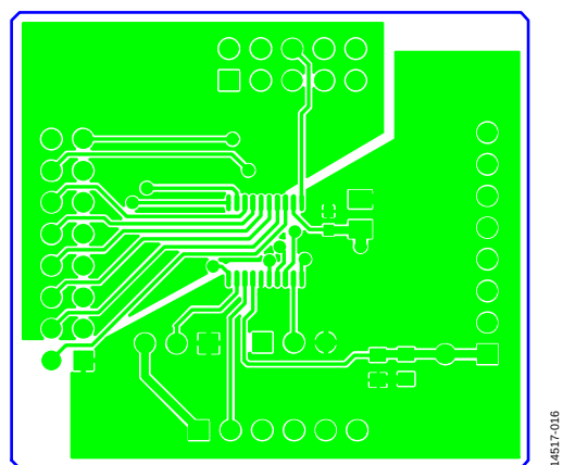
Figure 16. EVAL-AD5341DBZ Daughter Board Top Side Routing
