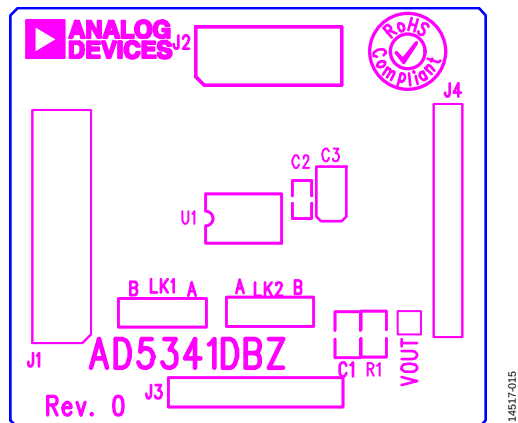
Figure 15. EVAL-AD5341DBZ Daughter Board Component Placement
