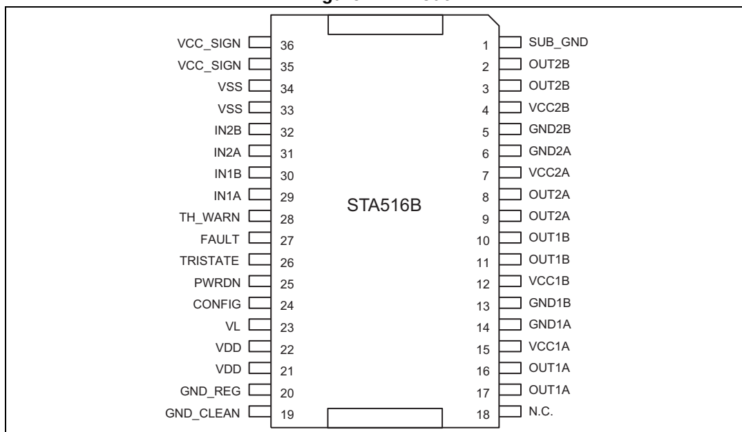
Figure 2. Pin out
