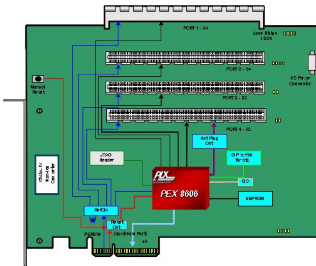
Figure 8. PEX 8606RDK
