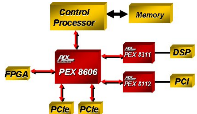
Figure 2. Fan-in/out Usage
