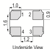
Underside View
