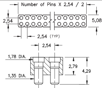
Coplanarity 0,13. For Pin Counts >20 positions consult Technical Support.
