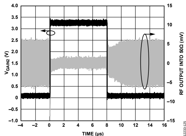
Figure 25. AMP2 Typical Output Response with 3.3 V Step on V_{\text{GAIN2}} , V_{\text{GAIN1}} = 3.3 V, HG Mode, 0.9 GHz
