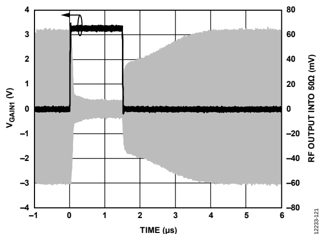
Figure 21. AMP2 Typical Output Response with 3.3 V Step on V_{\text{GAIN1}} , V_{\text{GAIN2}} = 0 V, HG Mode, 0.9 GHz
