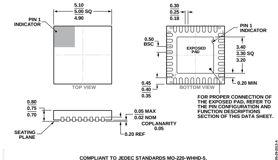
Figure 85. 32-Lead Lead Frame Chip Scale Package [LFCSP_WQ] 5 mm × 5 mm Body, Very Very Thin Quad (CP-32-20) Dimensions shown in millimeters
