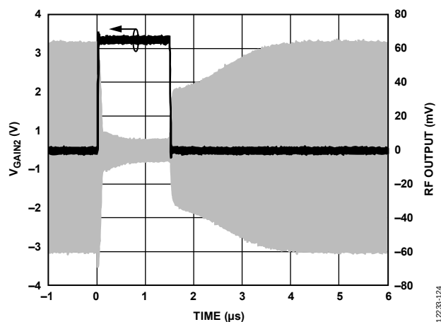
Figure 24. AMP2 Typical Output Response with 3.3 V Step on V_{\text{GAIN2}} , V_{\text{GAIN1}} = 0 V, HG Mode, 0.9 GHz
