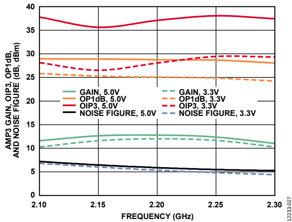
Figure 45. AMP3 2.2 GHz Gain, OIP3 at P_{OUT} = 0 dBm/Tone, OP1dB, and Noise Figure vs. Frequency
