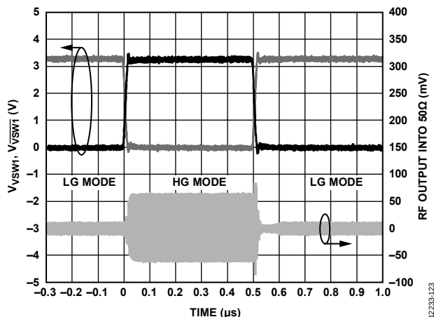
Figure 23. AMP2 Typical Output Response During Gain Mode Switching, V_{\text{GAIN1}} = V_{\text{GAIN2}} = 0 V, 0.9 GHz
