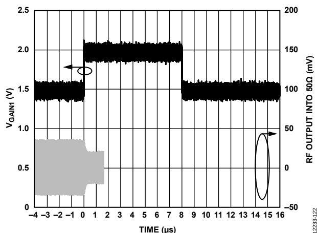
Figure 22. AMP2 Typical Output Response with 0.5 V Step on V_{\text{GAIN1}} , V_{\text{GAIN2}} = 0 V, HG Mode, 0.9 GHz
