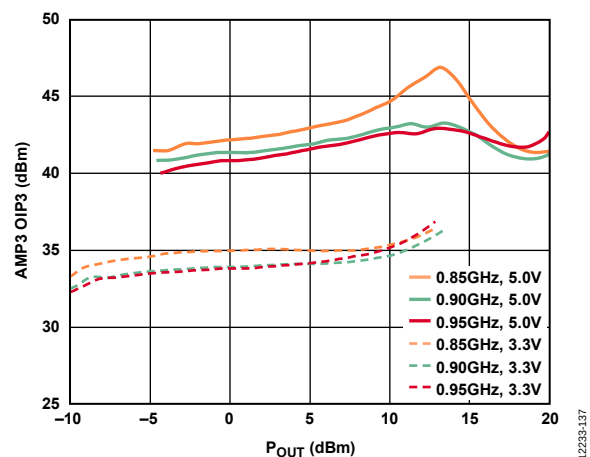
Figure 37. AMP3 0.9 GHz OIP3 vs. P_{OUT} by Frequency
