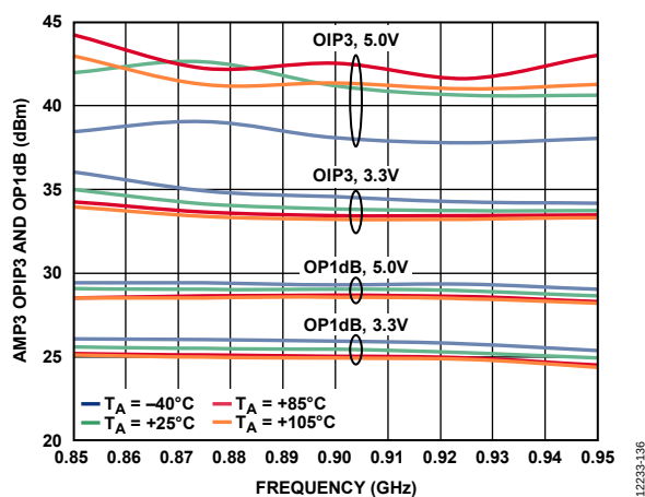
Figure 36. AMP3 0.9 GHz OIP3 at P_{OUT} = 0 dBm/Tone and OP1dB vs. Frequency by Temperature
