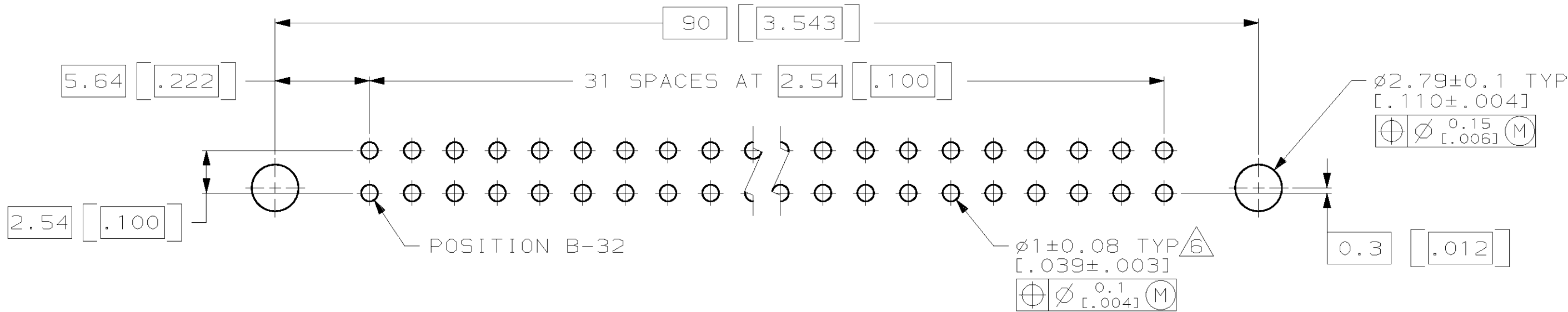
RECOMMENDED PC BOARD LAYOUT
