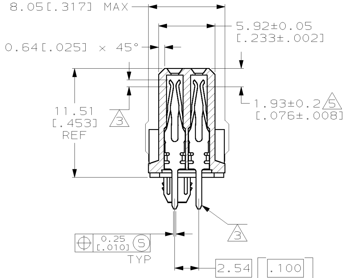
SECTION X-X
