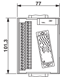
Dimensioned drawing
